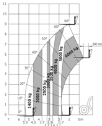
Industrial load chart standard EN1459 B Machines on tyres with forks
